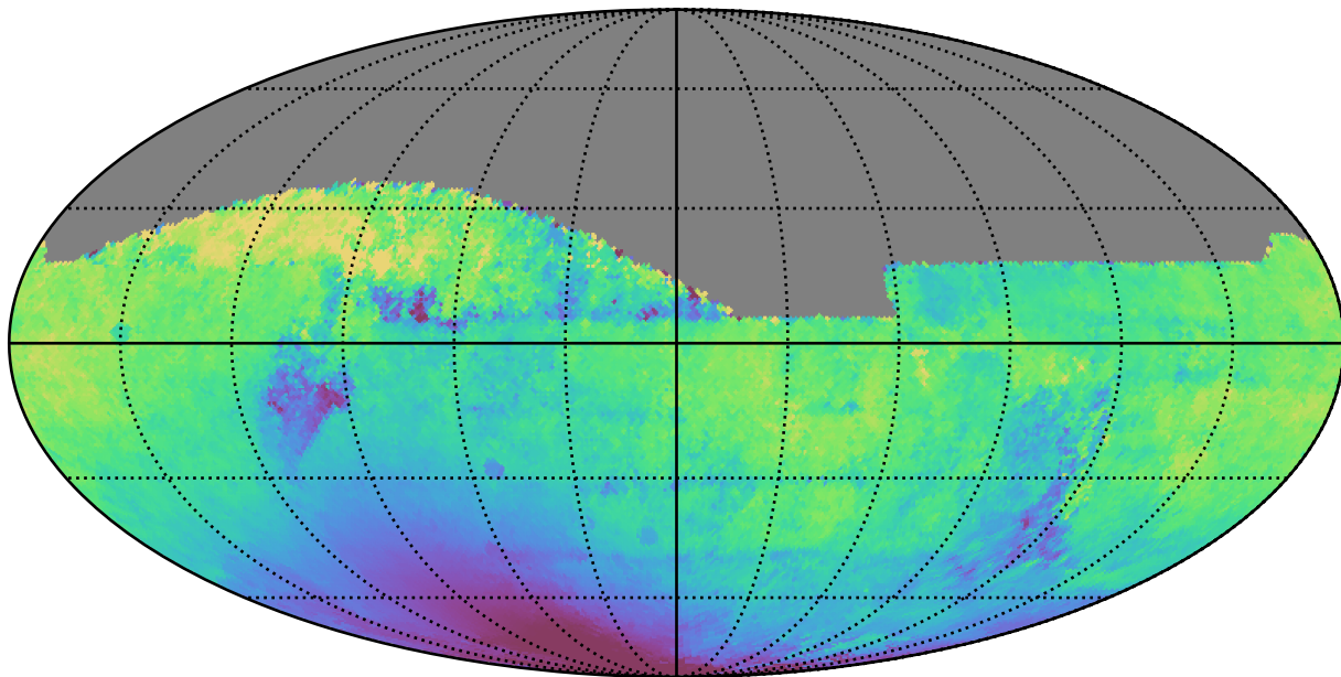
early_u_fpextra2.0_v3.4_10yrs All sky z band: Median solarElong
