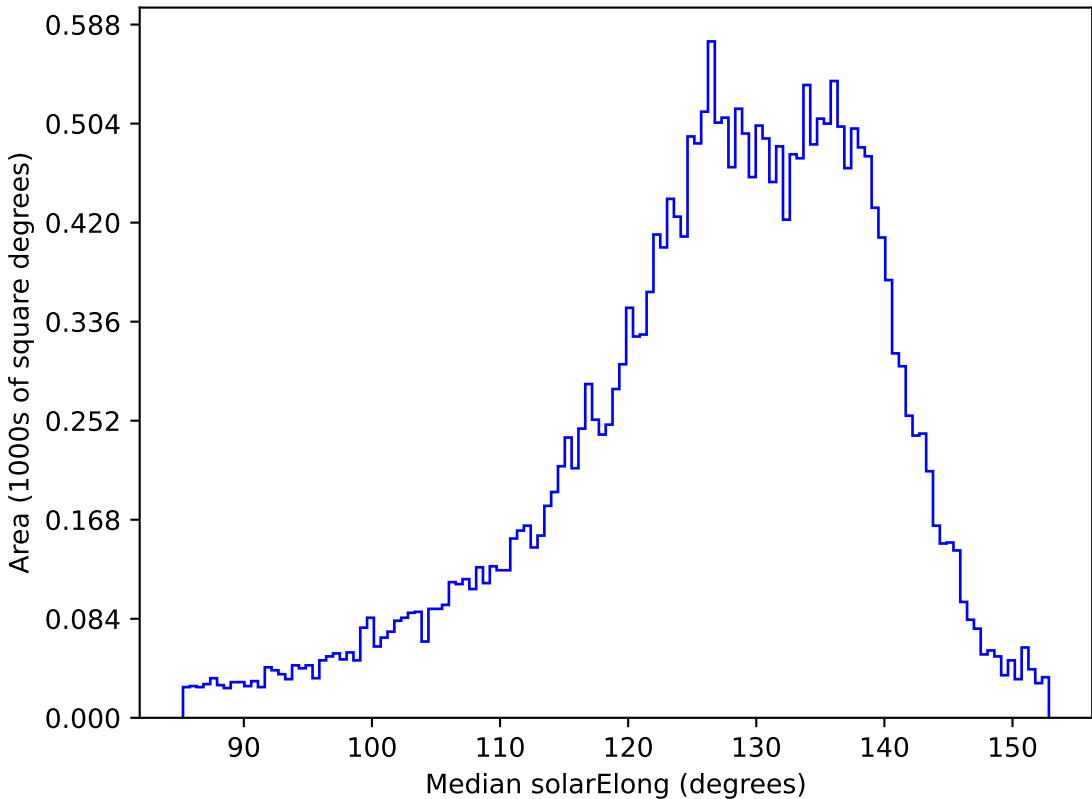
early_u_fpextra2.0_v3.4_10yrs All sky z band: Median solarElong
