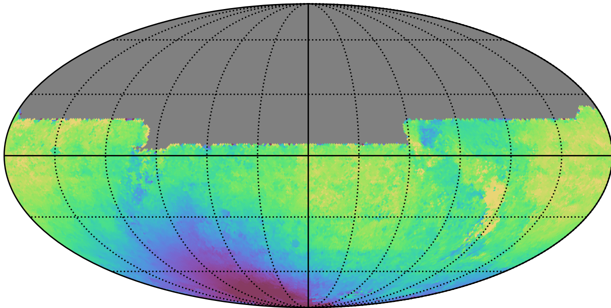
early_u_fpextra2.0_v3.4_10yrs All sky y band: Median solarElong
