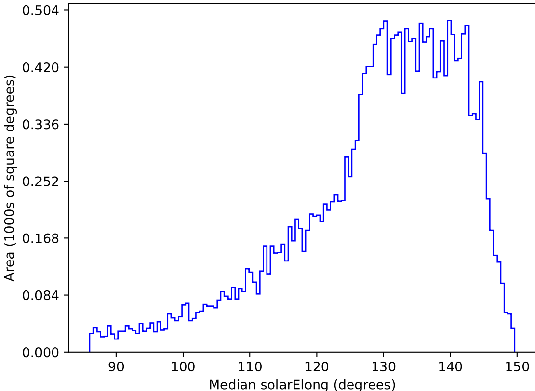
early_u_fpextra2.0_v3.4_10yrs All sky y band: Median solarElong
