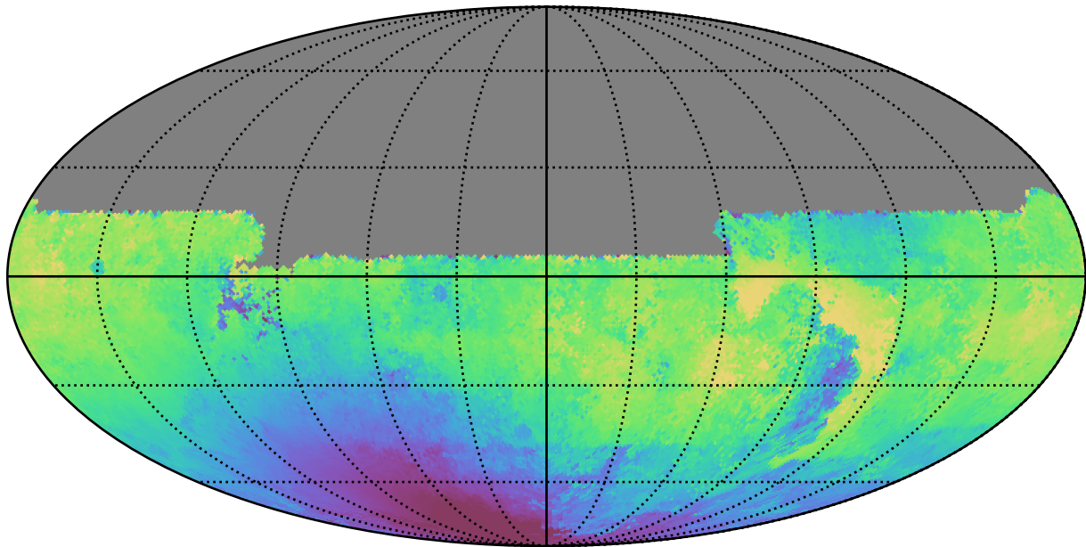
early_u_fpextra2.0_v3.4_10yrs All sky u band: Median solarElong
