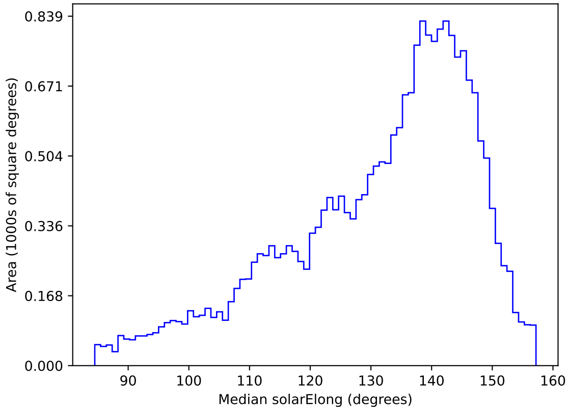
early_u_fpextra2.0_v3.4_10yrs All sky u band: Median solarElong
