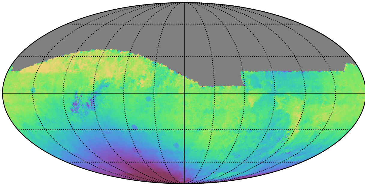
early_u_fpextra2.0_v3.4_10yrs All sky r band: Median solarElong
