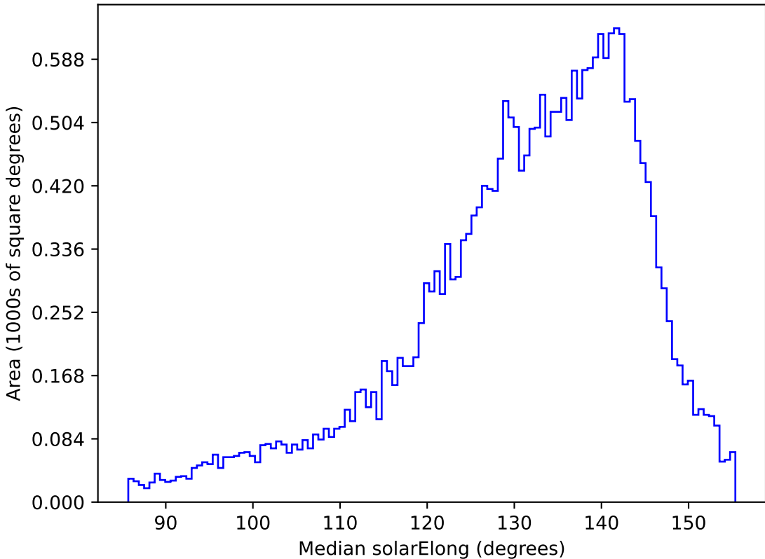
early_u_fpextra2.0_v3.4_10yrs All sky r band: Median solarElong
