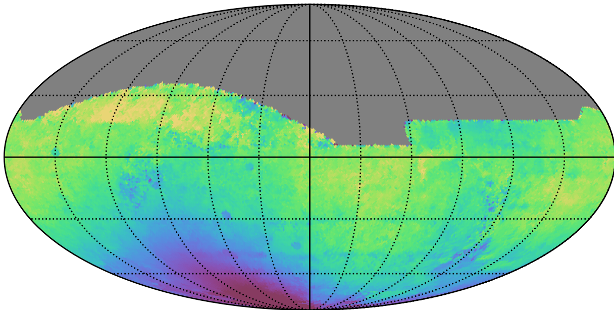
early_u_fpextra2.0_v3.4_10yrs All sky i band: Median solarElong
