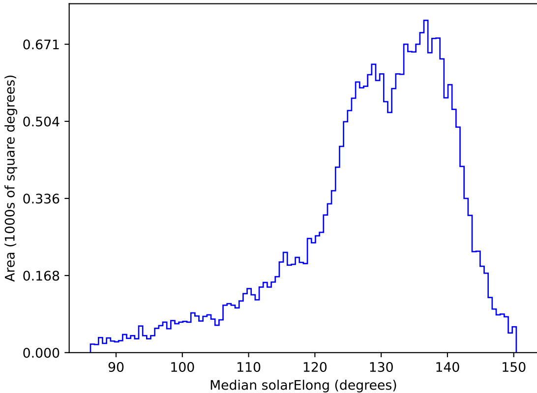
early_u_fpextra2.0_v3.4_10yrs All sky i band: Median solarElong
