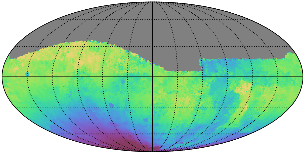
early_u_fpextra2.0_v3.4_10yrs All sky g band: Median solarElong
