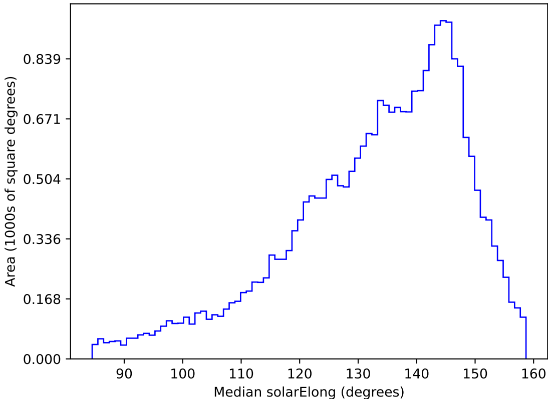
early_u_fpextra2.0_v3.4_10yrs All sky g band: Median solarElong
