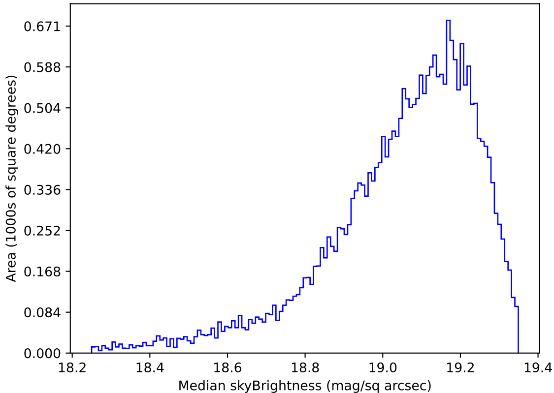
early_u_fpxextra2.0_v3.4_10yrs Yr 1 z band: Median skyBrightness
