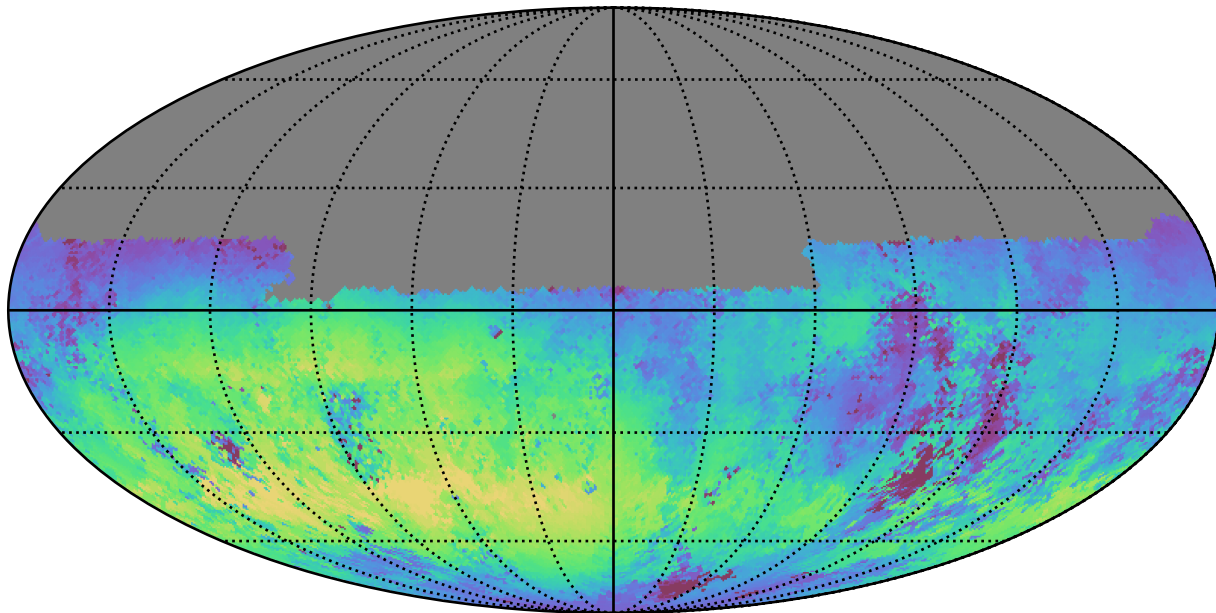
early_u_fpextra2.0_v3.4_10yrs Yr 1 u band: Median skyBrightness
