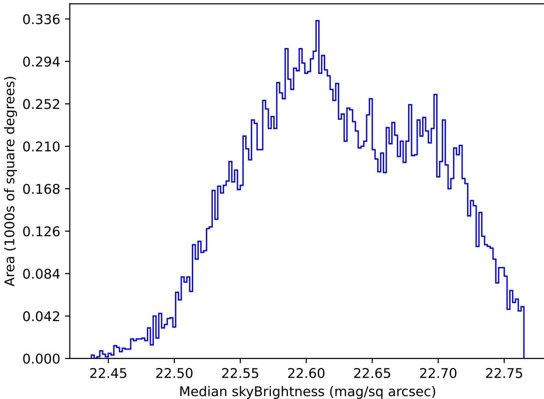
early_u_fpextra2.0_v3.4_10yrs Yr 1 u band: Median skyBrightness
