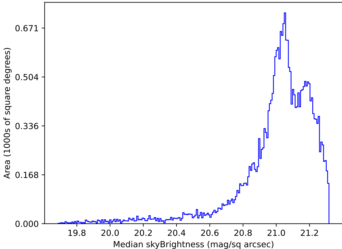
early_u_fpextra2.0_v3.4_10yrs Yr 1 r band: Median skyBrightness
