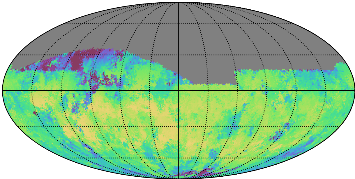
early_u_fpextra2.0_v3.4_10yrs Yr 1 i band: Median skyBrightness
