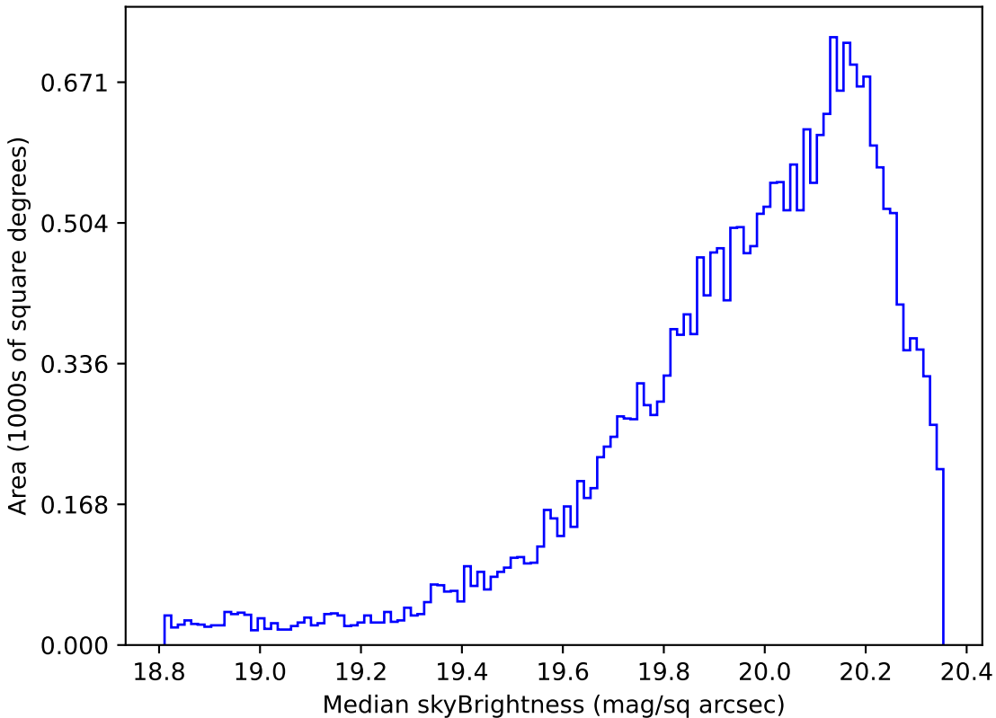
early_u_fpextra2.0_v3.4_10yrs Yr 1 i band: Median skyBrightness
