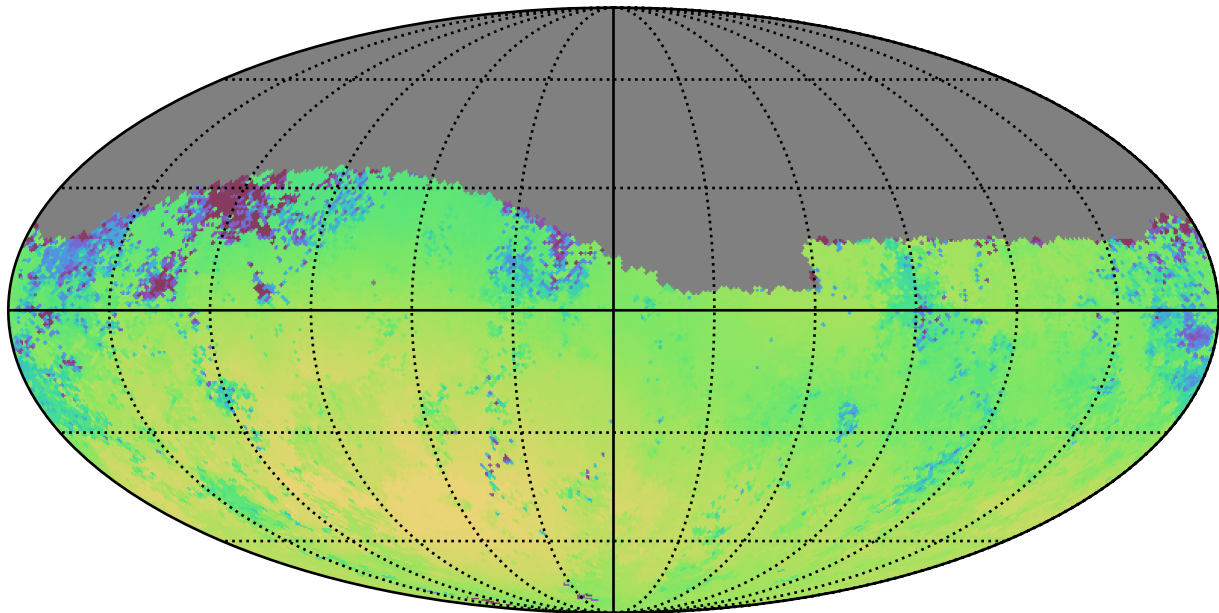
early_u_fpextra2.0_v3.4_10yrs Yr 1 g band: Median skyBrightness
