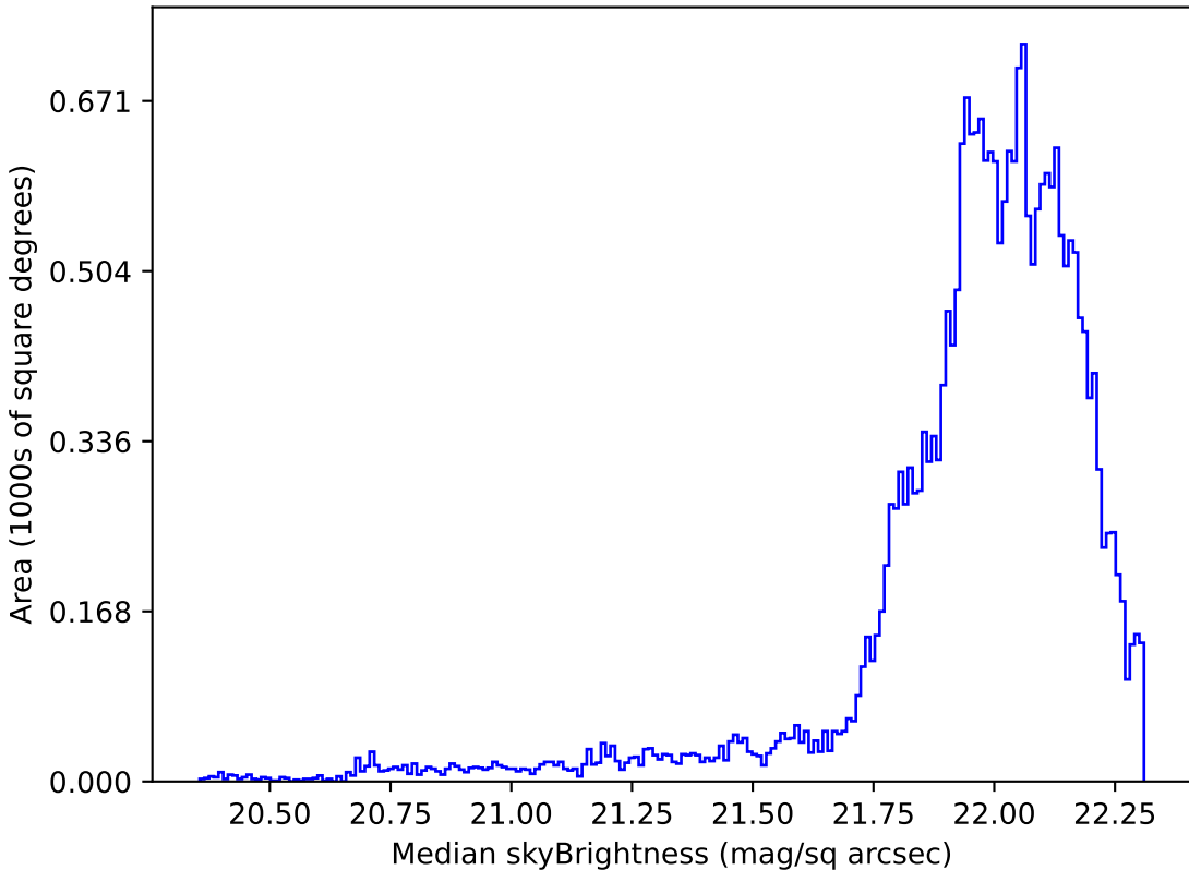
early_u_fpextra2.0_v3.4_10yrs Yr 1 g band: Median skyBrightness
