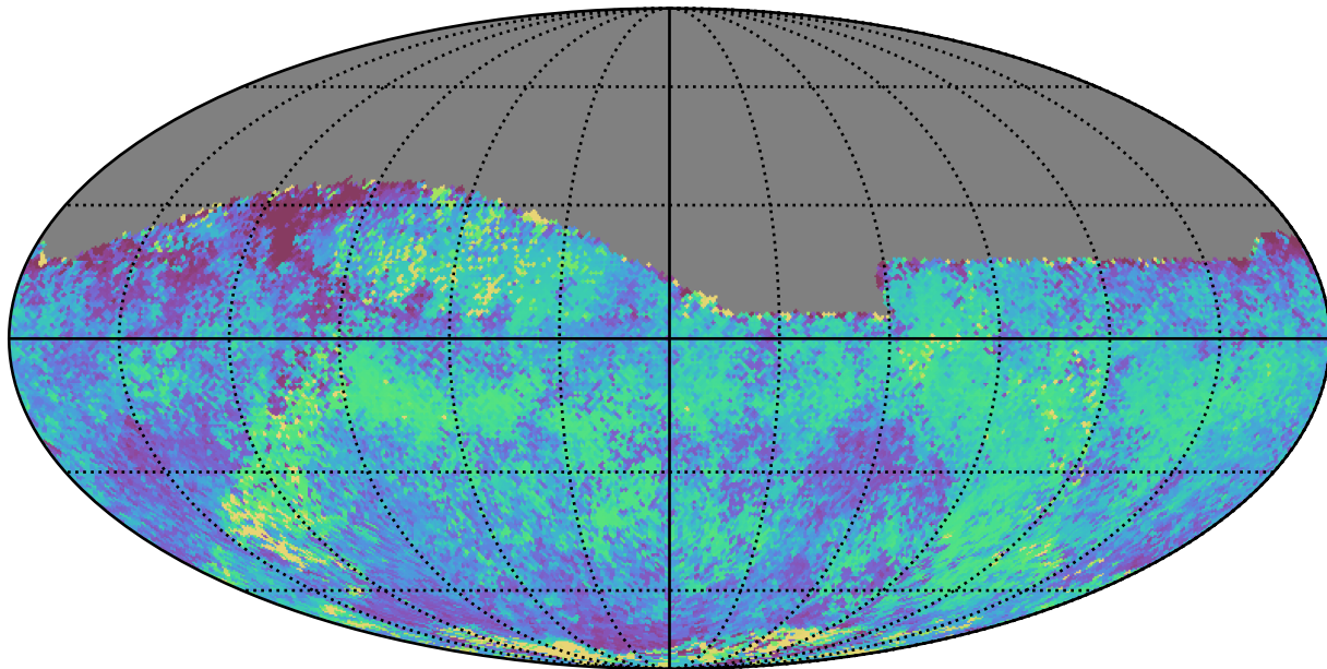
early_u_fpextra2.0_v3.4_10yrs Yr 1 all bands: Median skyBrightness
