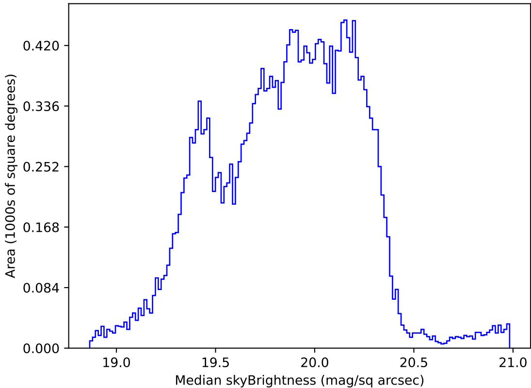
early_u_fpextra2.0_v3.4_10yrs Yr 1 all bands: Median skyBrightness
