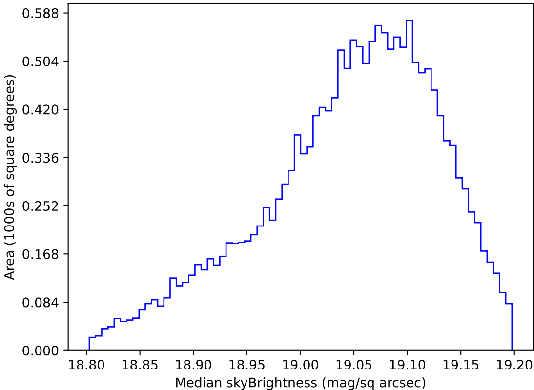
early_u_fpextra2.0_v3.4_10yrs WFD z band: Median skyBrightness
