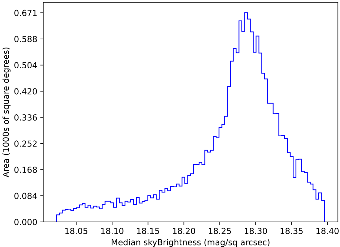
early_u_fpextra2.0_v3.4_10yrs WFD y band: Median skyBrightness
