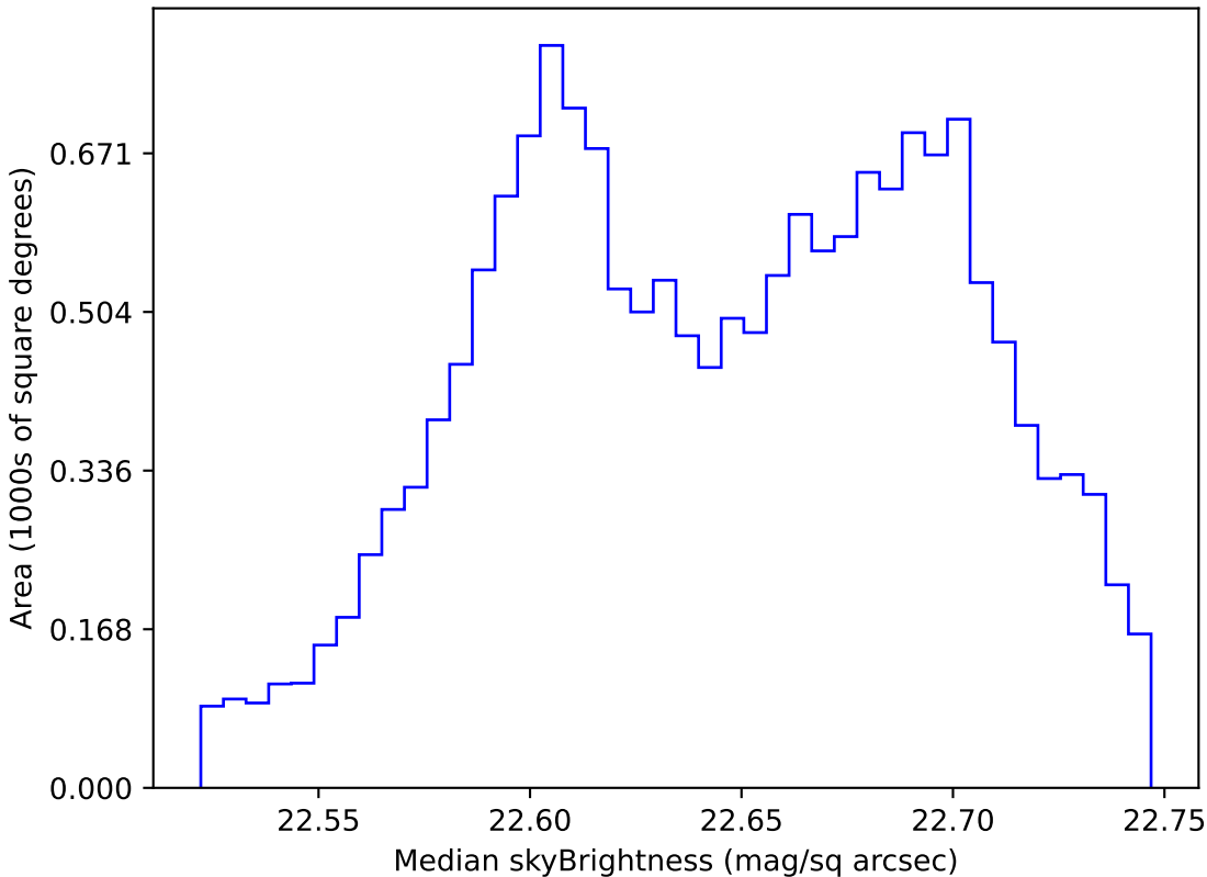
early_u_fpextra2.0_v3.4_10yrs WFD u band: Median skyBrightness
