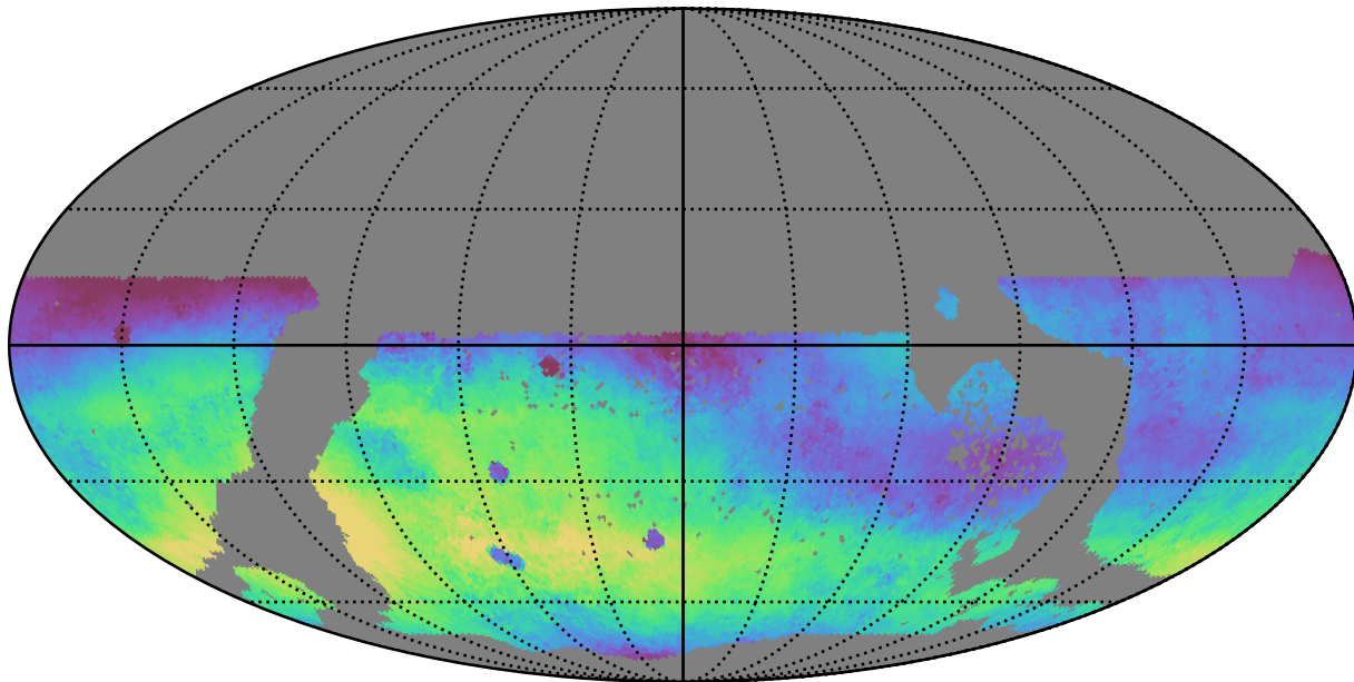
early_u_fpextra2.0_v3.4_10yrs WFD r band: Median skyBrightness
