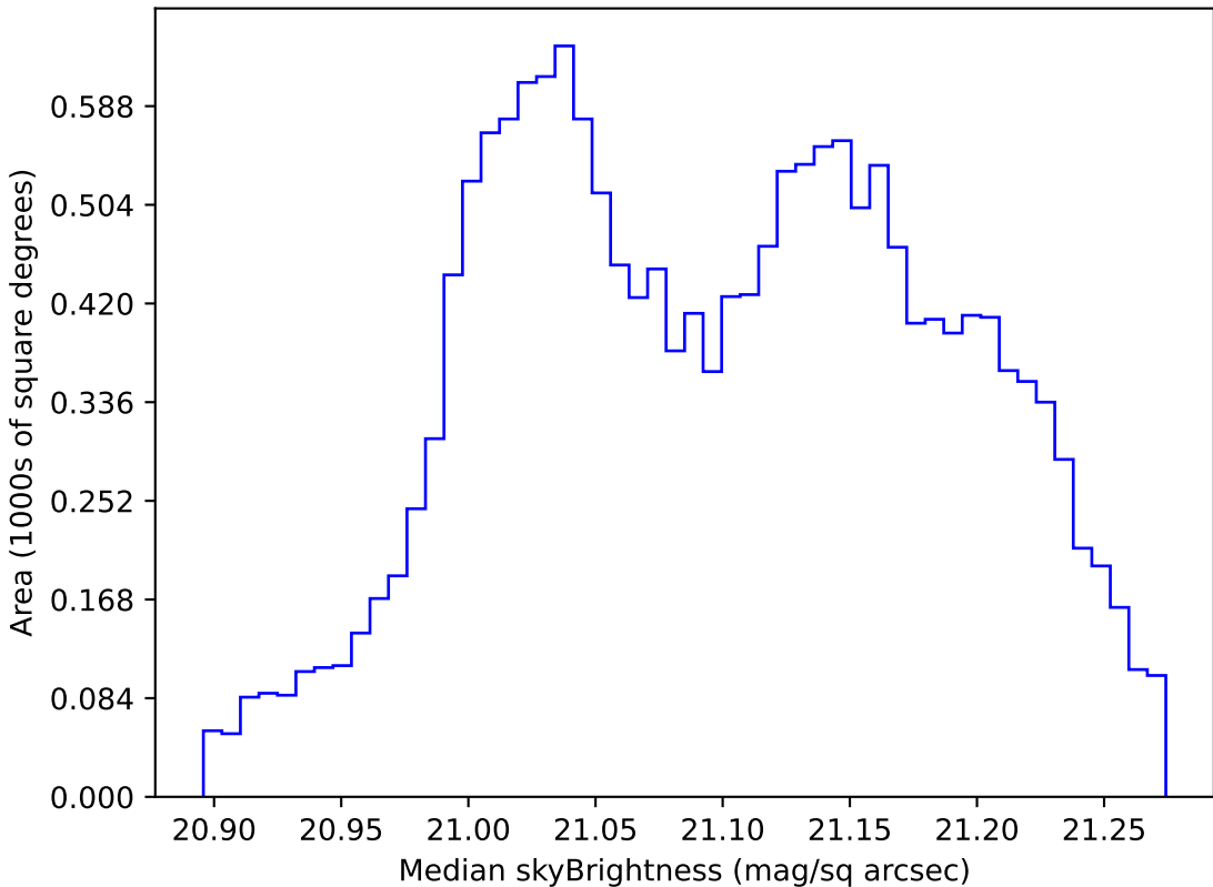
early_u_fpextra2.0_v3.4_10yrs WFD r band: Median skyBrightness
