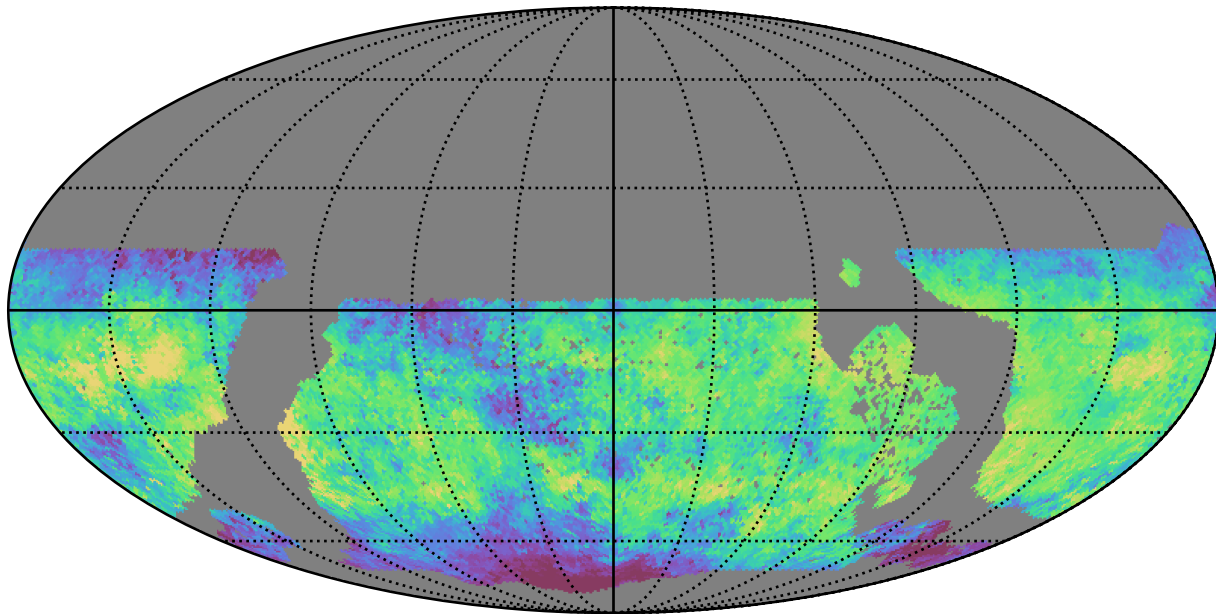
early_u_fpextra2.0_v3.4_10yrs WFD i band: Median skyBrightness
