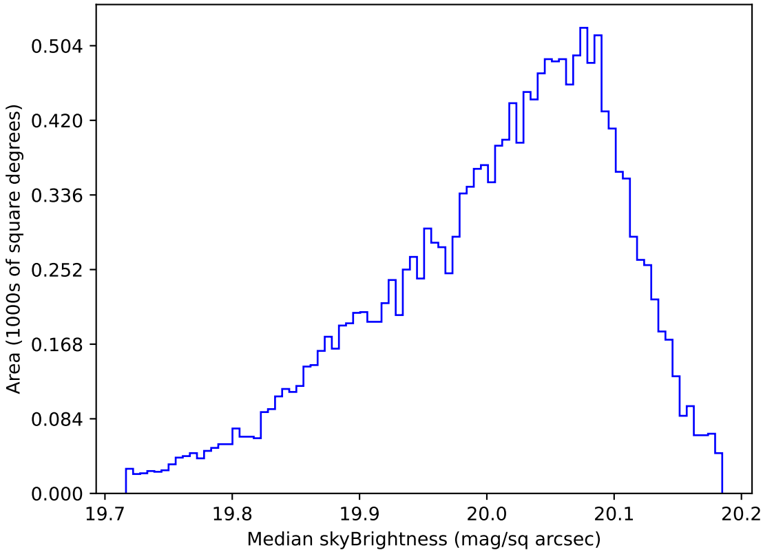
early_u_fpextra2.0_v3.4_10yrs WFD i band: Median skyBrightness
