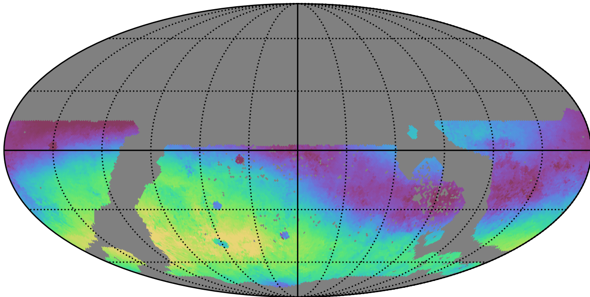
early_u_fpextra2.0_v3.4_10yrs WFD g band: Median skyBrightness
