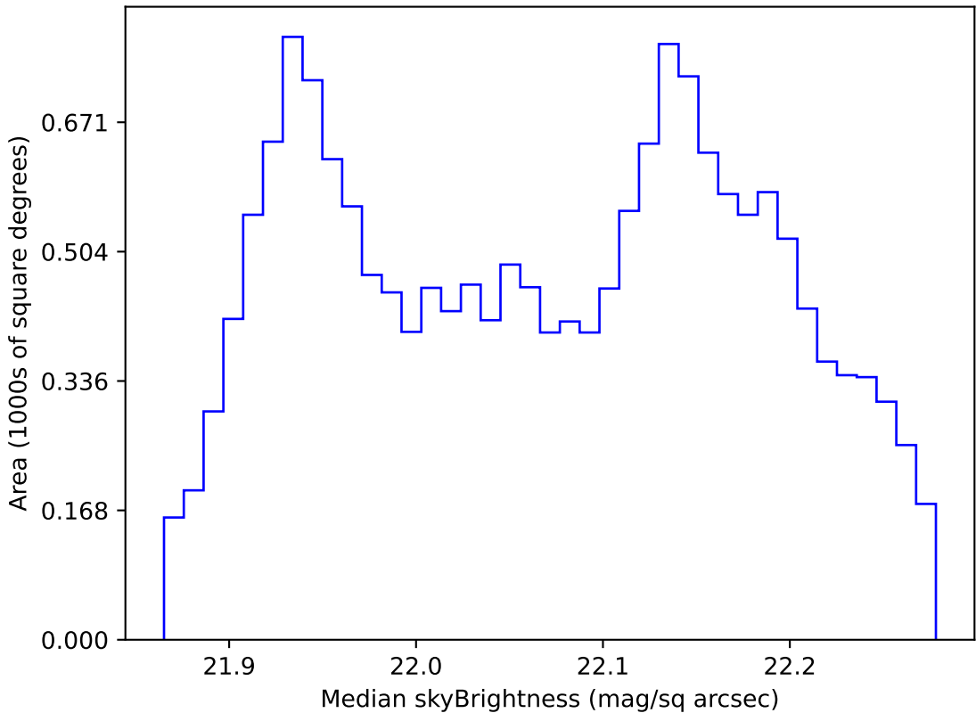
early_u_fpextra2.0_v3.4_10yrs WFD g band: Median skyBrightness
