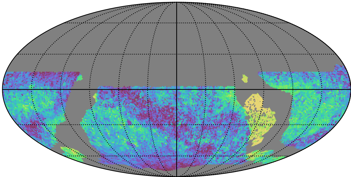
early_u_fpextra2.0_v3.4_10yrs WFD all bands: Median skyBrightness
