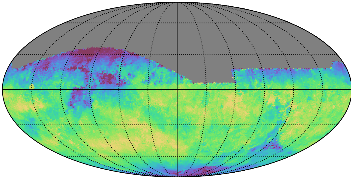
early_u_fpextra2.0_v3.4_10yrs All sky z band: Median skyBrightness
