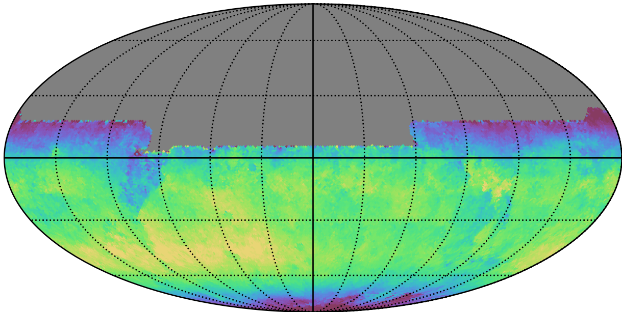
early_u_fpextra2.0_v3.4_10yrs All sky y band: Median skyBrightness
