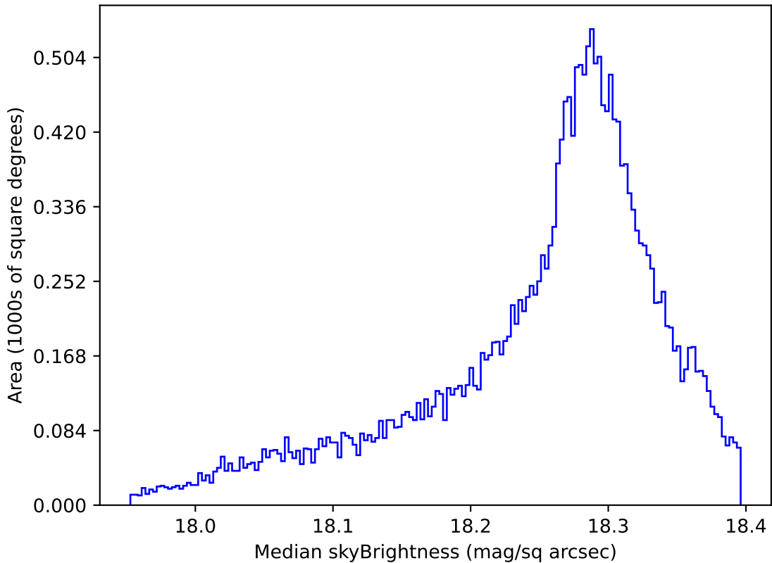
early_u_fpextra2.0_v3.4_10yrs All sky y band: Median skyBrightness
