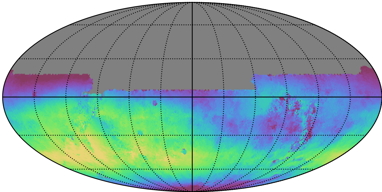
early_u_fpextra2.0_v3.4_10yrs All sky u band: Median skyBrightness
