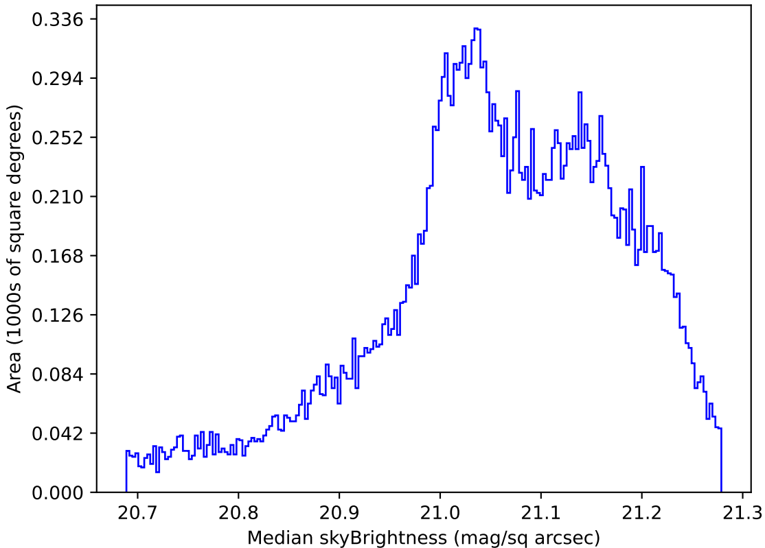
early_u_fpextra2.0_v3.4_10yrs All sky r band: Median skyBrightness
