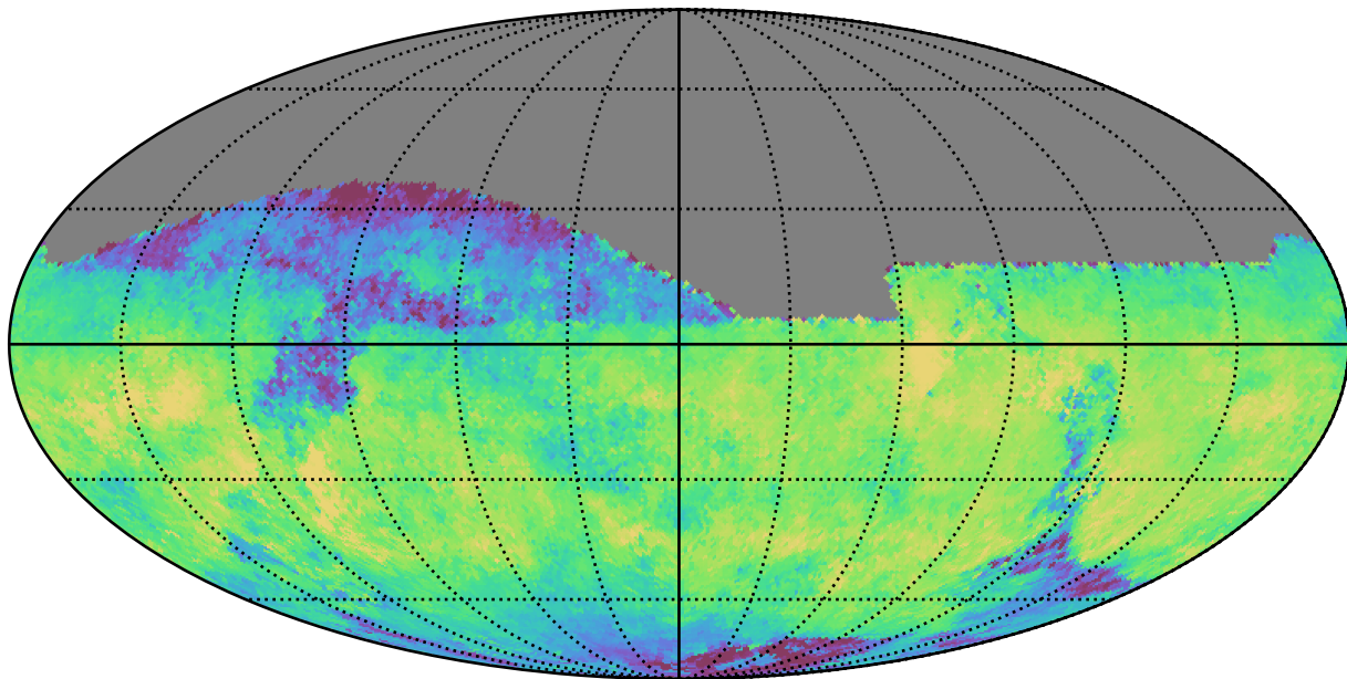
early_u_fpextra2.0_v3.4_10yrs All sky i band: Median skyBrightness
