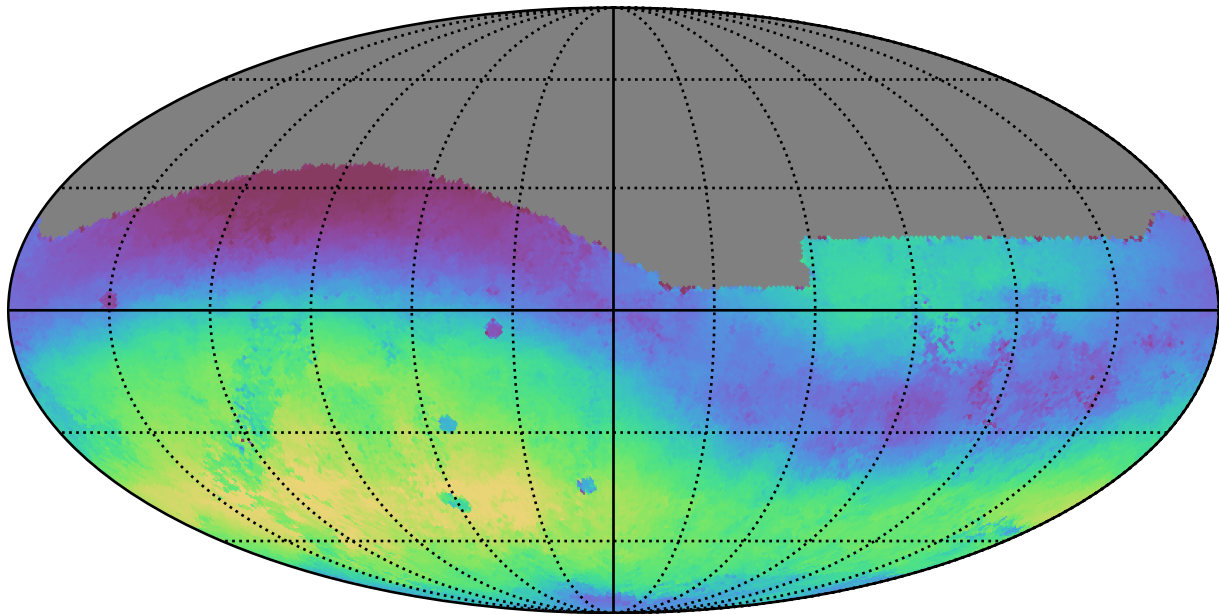
early_u_fpextra2.0_v3.4_10yrs All sky g band: Median skyBrightness
