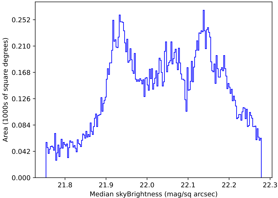
early_u_fpextra2.0_v3.4_10yrs All sky g band: Median skyBrightness
