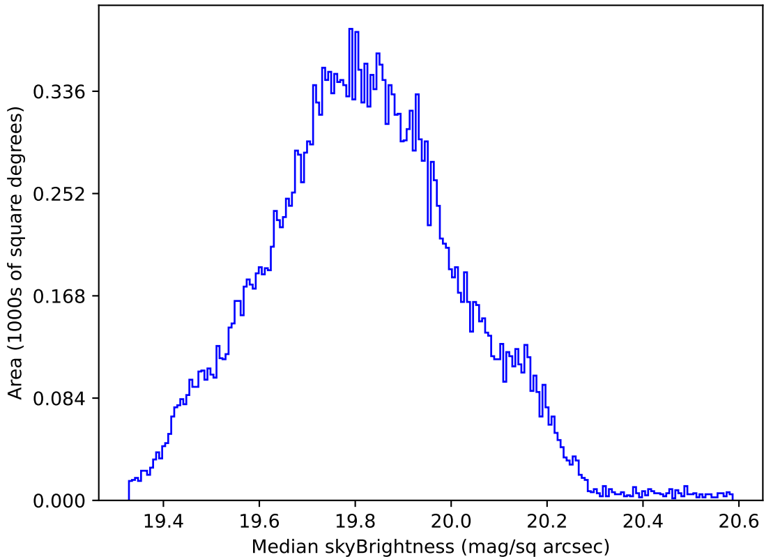
early_u_fpextra2.0_v3.4_10yrs All sky all bands: Median skyBrightness
