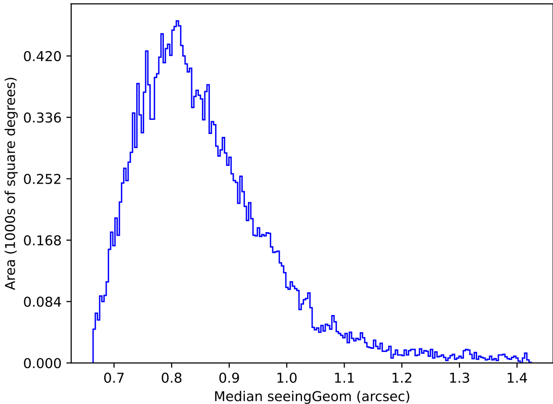
early_u_fpextra2.0_v3.4_10yrs Yr 1 z band: Median seeingGeom
