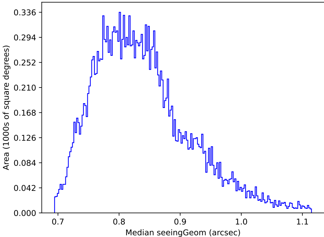
early_u_fpextra2.0_v3.4_10yrs Yr 1 y band: Median seeingGeom
