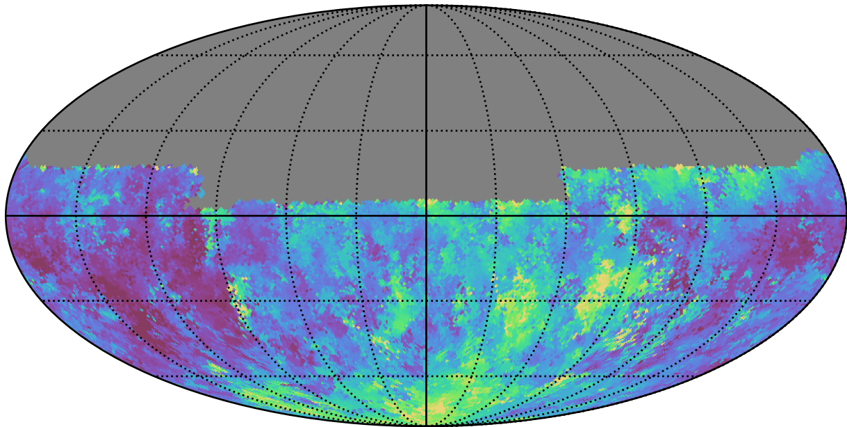
early_u_fpextra2.0_v3.4_10yrs Yr 1 u band: Median seeingGeom
