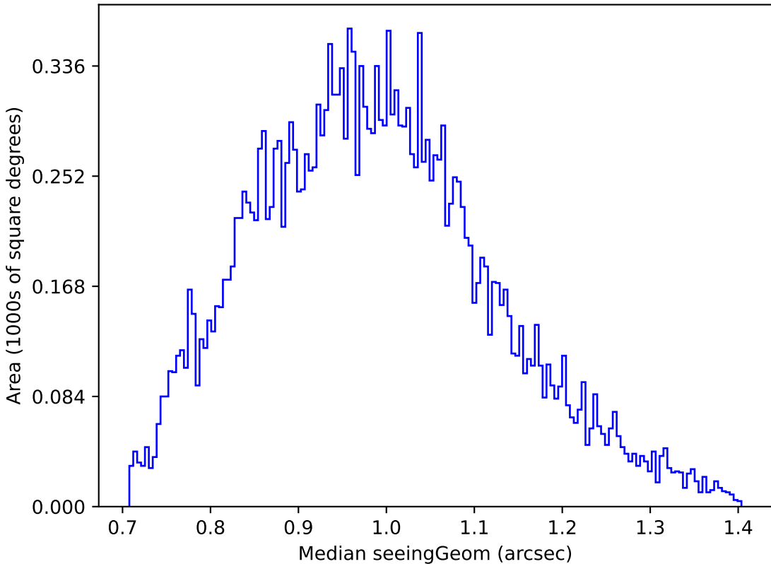
early_u_fpextra2.0_v3.4_10yrs Yr 1 u band: Median seeingGeom
