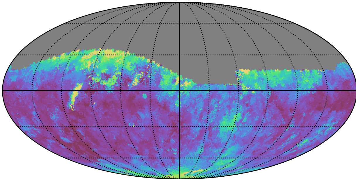
early_u_fpextra2.0_v3.4_10yrs Yr 1 r band: Median seeingGeom
