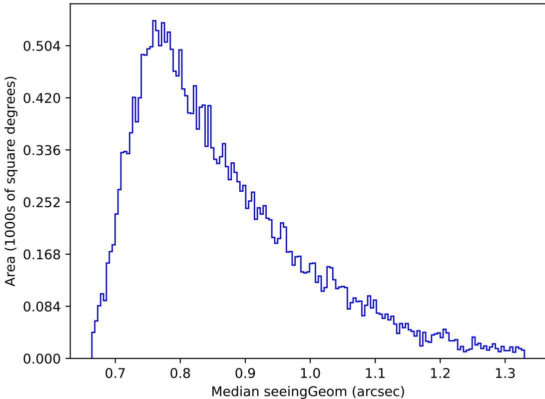
early_u_fpextra2.0_v3.4_10yrs Yr 1 r band: Median seeingGeom
