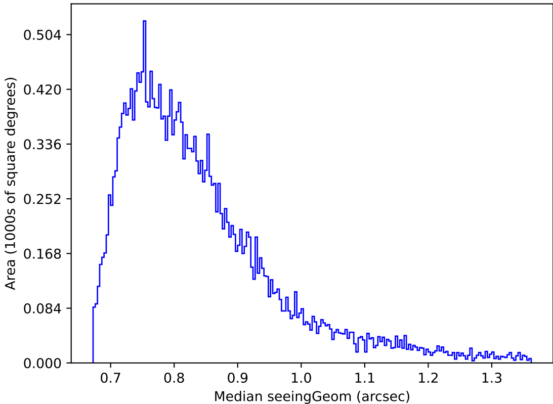
early_u_fpextra2.0_v3.4_10yrs Yr 1 i band: Median seeingGeom
