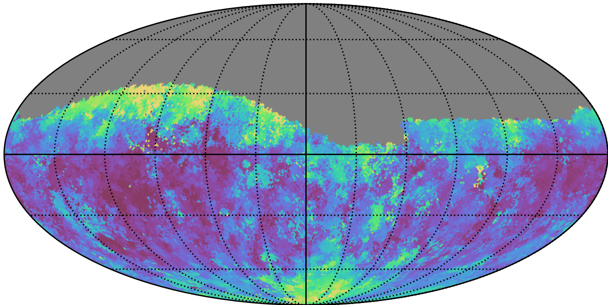
early_u_fpextra2.0_v3.4_10yrs Yr 1 g band: Median seeingGeom
