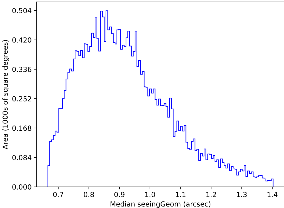
early_u_fpextra2.0_v3.4_10yrs Yr 1 g band: Median seeingGeom
